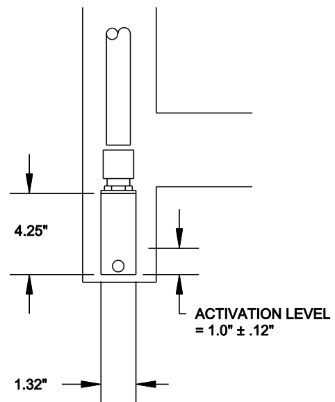
PSTV FLOAT SWITCH ASSEMBLY DETAIL
